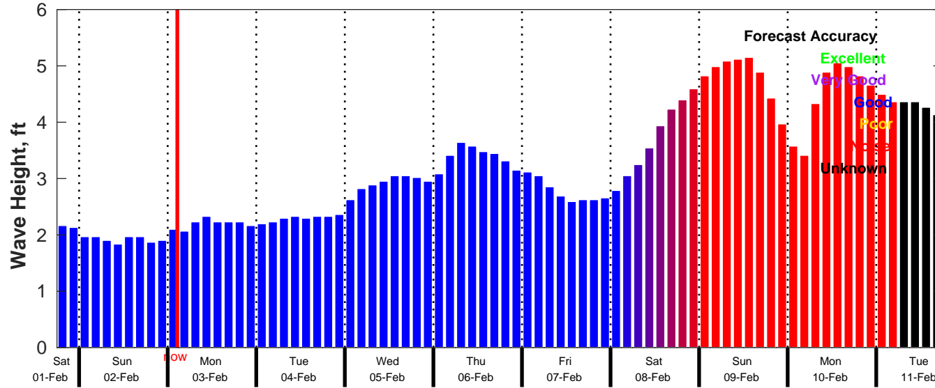
CMEMS Wave Forecast for NDBC 42019 from 01-Feb-2025 18:00:00 to 11-Feb-2025 18:00:00
