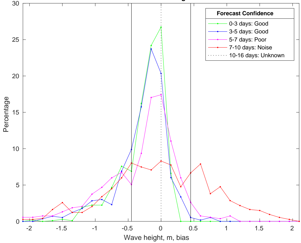
NDBC 42020 vs CMEMSWaves Bias Histogram: 03-Feb-2025
