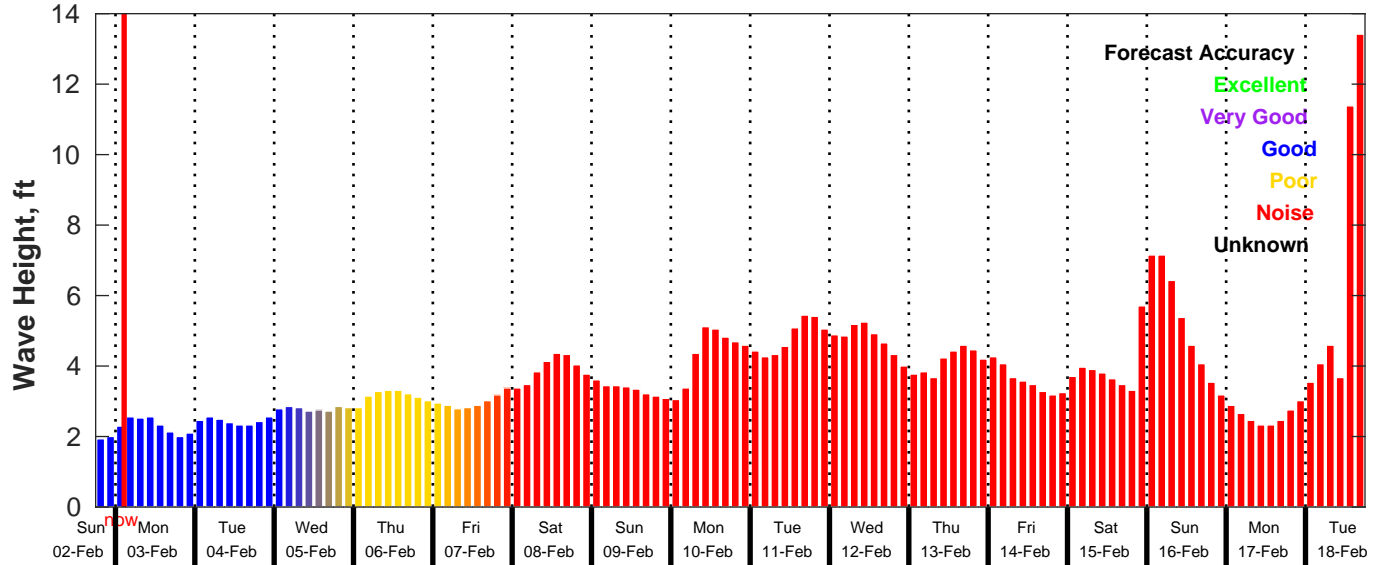
GFS Wave Forecast for NDBC 42020 from 02-Feb-2025 18:00:00 to 18-Feb-2025 18:00:00
