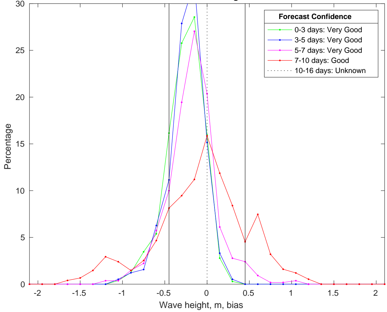
NDBC 42035 vs CMEMSWaves Bias Histogram: 03-Feb-2025
