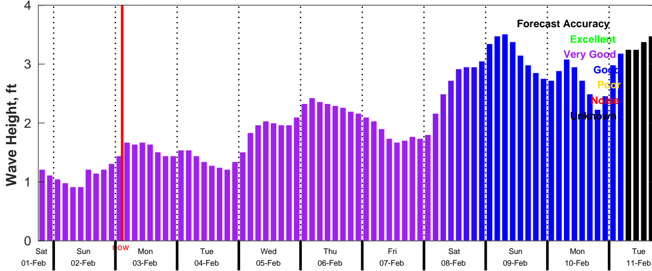
CMEMS Wave Forecast for NDBC 42035 from 01-Feb-2025 18:00:00 to 11-Feb-2025 18:00:00
