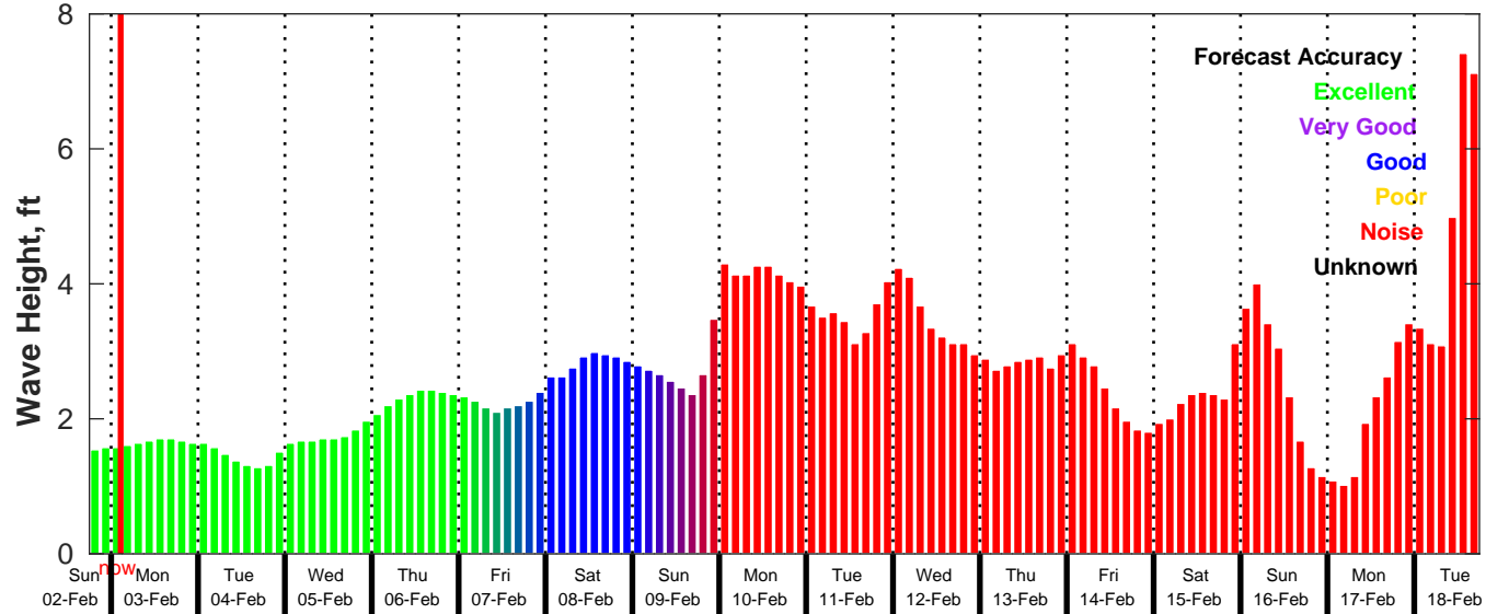
GFS Wave Forecast for NDBC 42035 from 02-Feb-2025 18:00:00 to 18-Feb-2025 18:00:00
