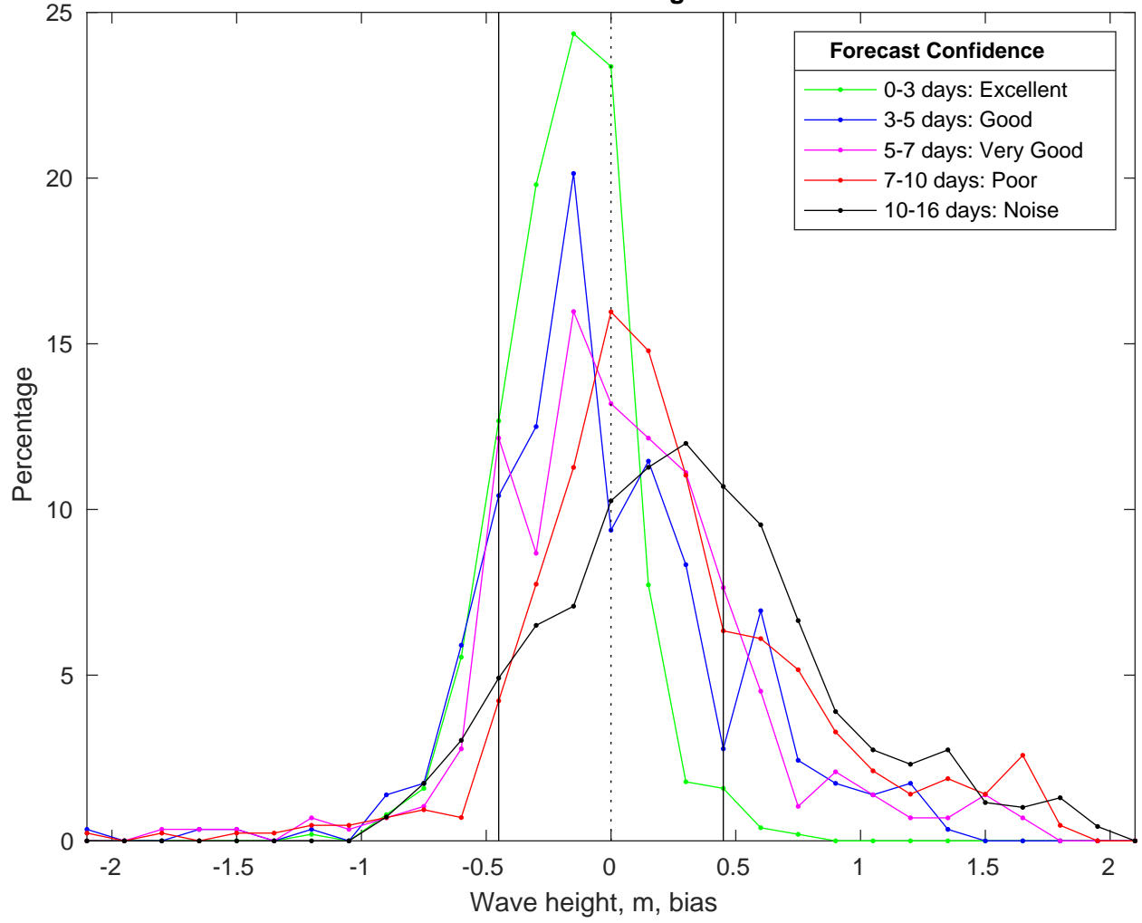
NDBC 42036 vs GFSWaves Bias Histogram: 03-Feb-2025
