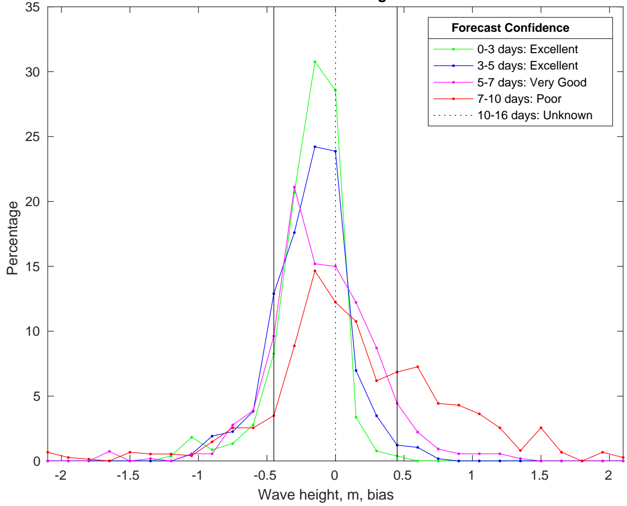
NDBC 42040 vs CMEMSWaves Bias Histogram: 03-Feb-2025
