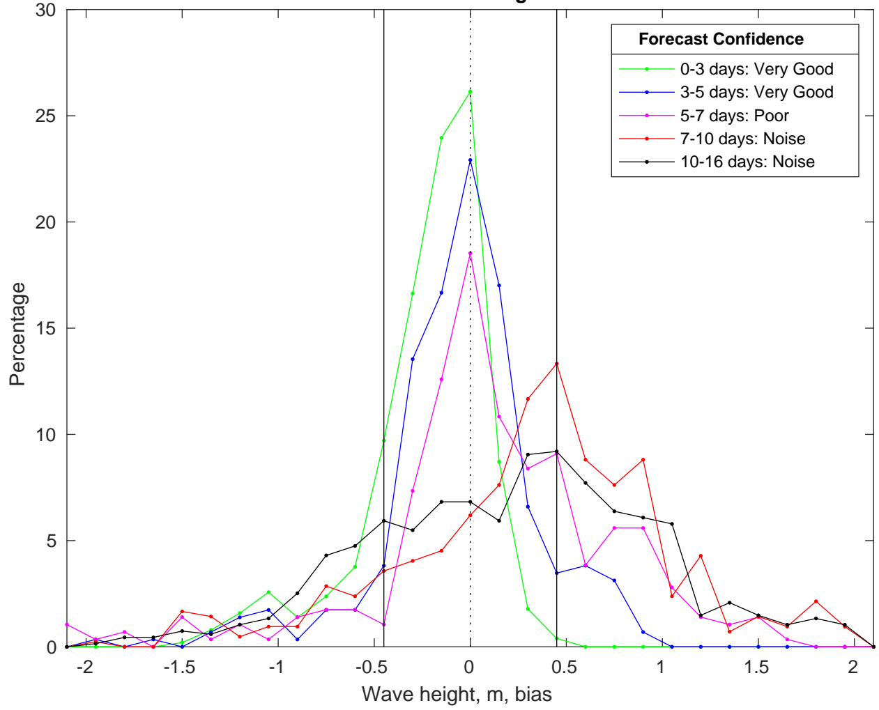
NDBC 42040 vs GFSWaves Bias Histogram: 03-Feb-2025
