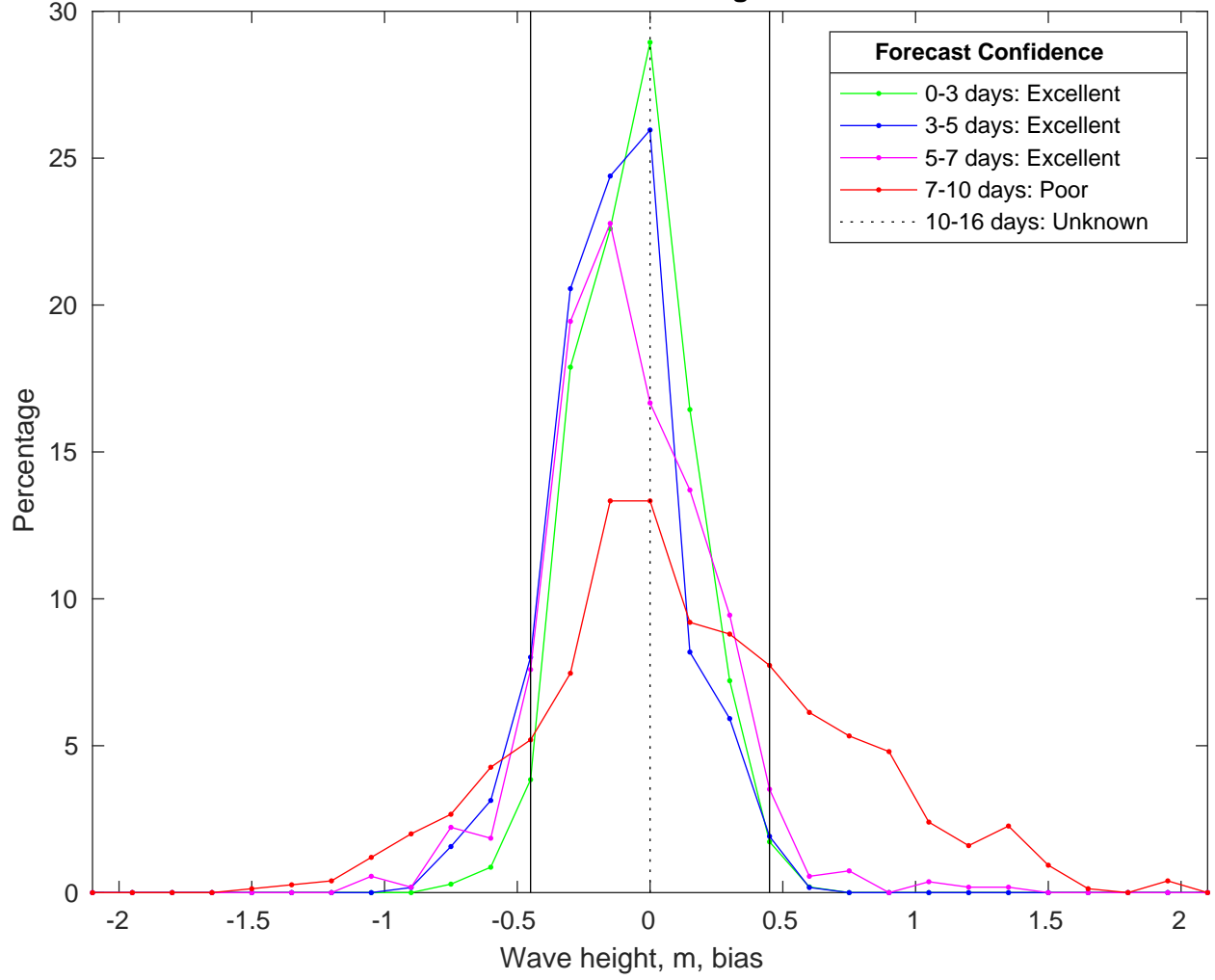
NDBC 42084 vs CMEMSWaves Bias Histogram: 03-Feb-2025
