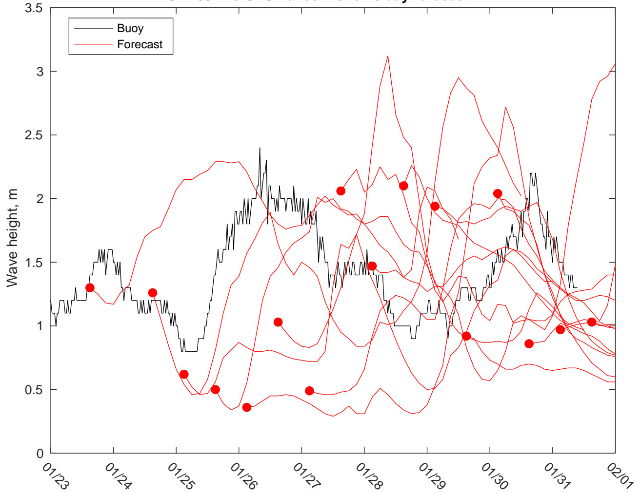
NDBC 42092 vs GFSWaves: 10 to 16 day forecast
