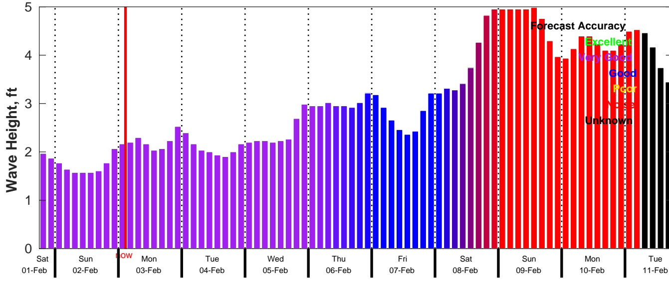
CMEMS Wave Forecast for NDBC 42092 from 01-Feb-2025 18:00:00 to 11-Feb-2025 18:00:00
