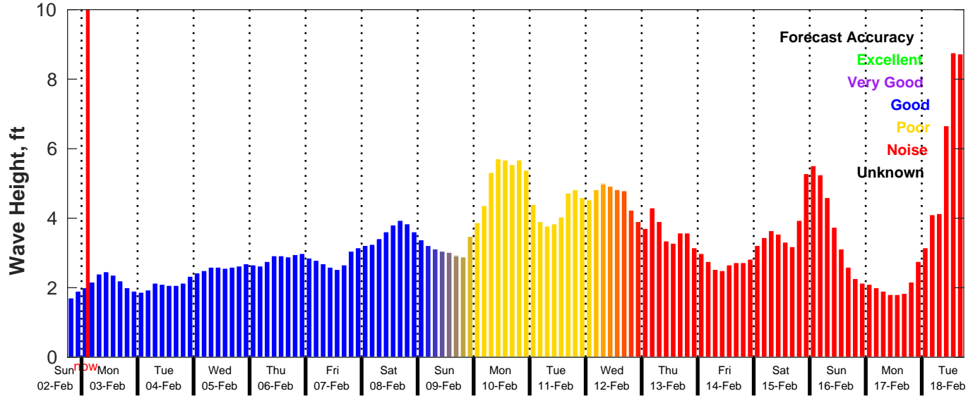
GFS Wave Forecast for NDBC 42092 from 02-Feb-2025 18:00:00 to 18-Feb-2025 18:00:00
