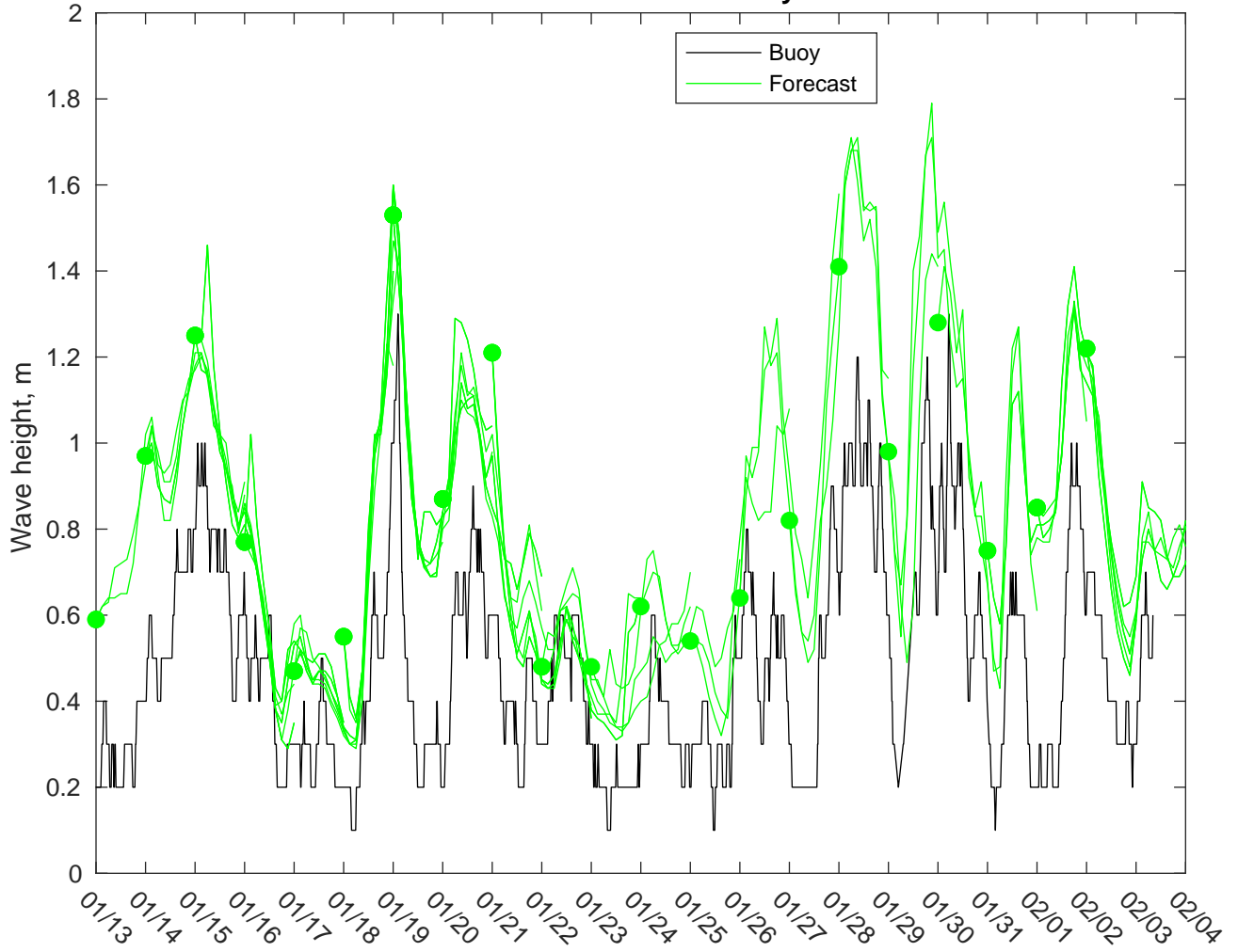
NDBC 44020 vs CMEMSWaves: 0 to 3 day forecast
