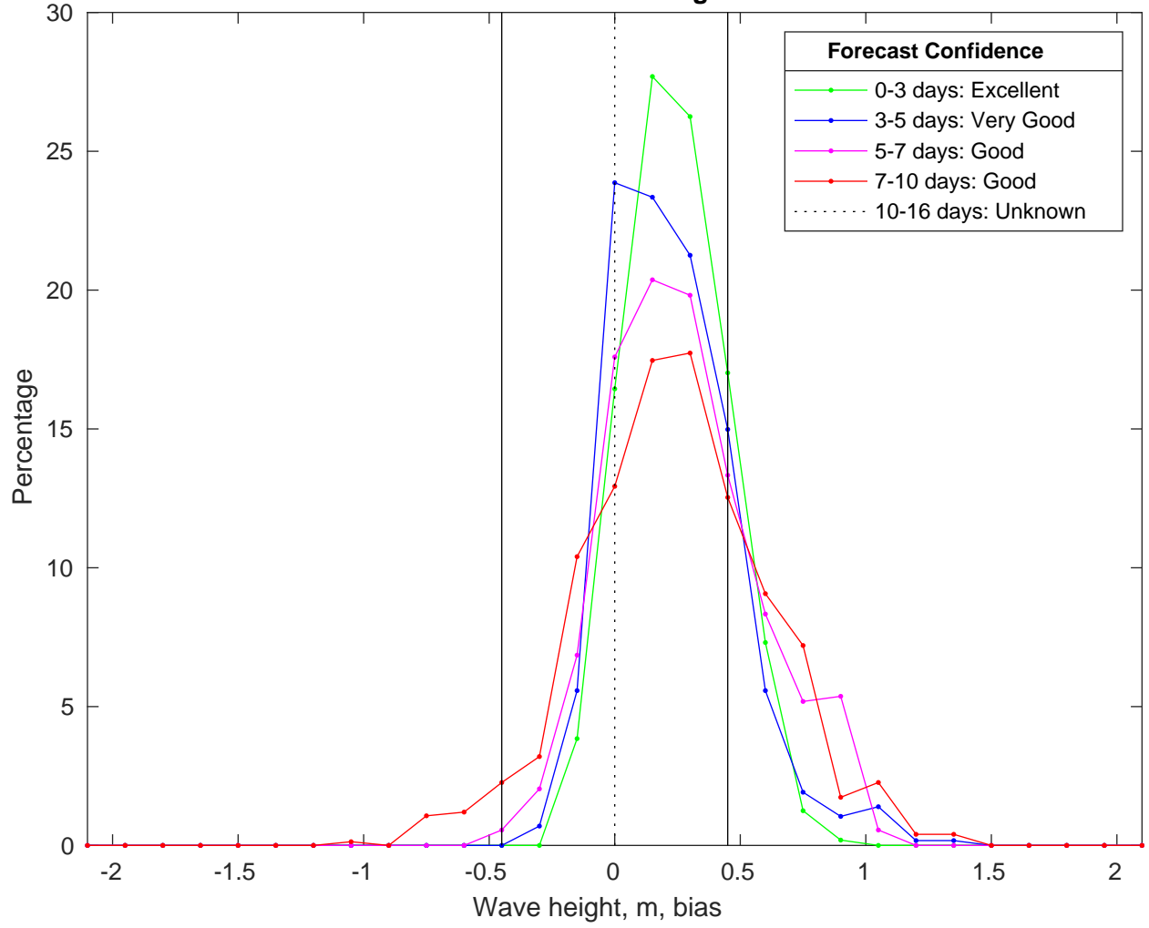
NDBC 44020 vs CMEMSWaves Bias Histogram: 03-Feb-2025
