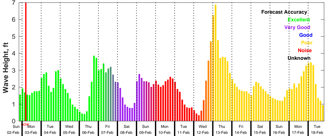
GFS Wave Forecast for NDBC 44020 from 02-Feb-2025 20:00:00 to 18-Feb-2025 20:00:00
