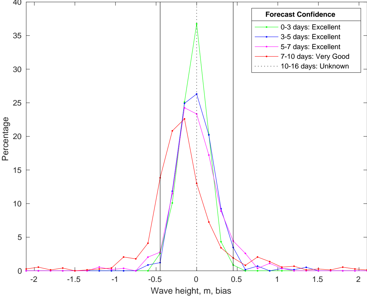
NDBC 46011 vs CMEMSWaves Bias Histogram: 03-Feb-2025
