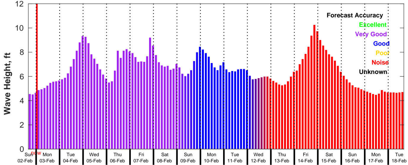
GFS Wave Forecast for NDBC 46011 from 02-Feb-2025 16:00:00 to 18-Feb-2025 16:00:00
