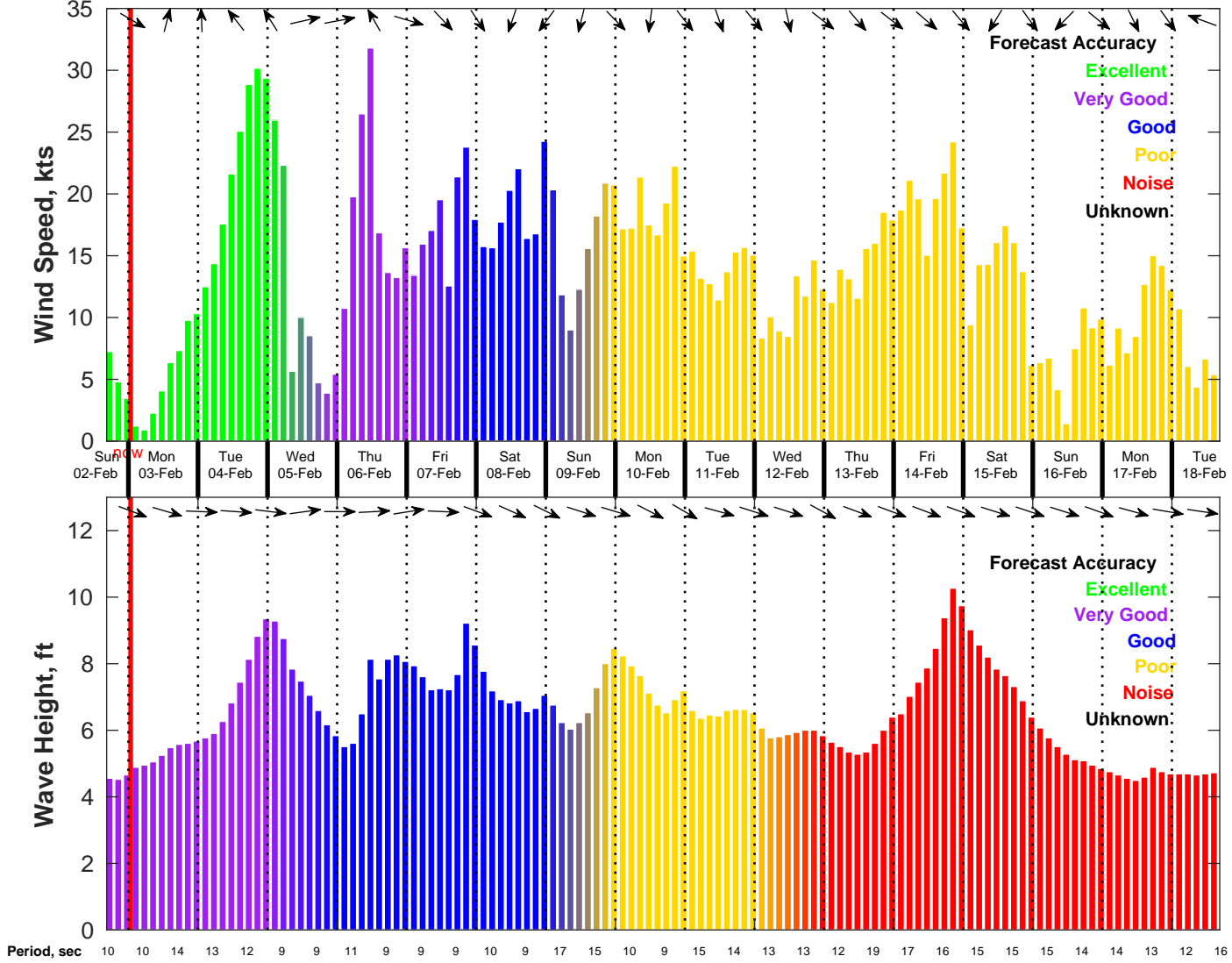
Wind & Wave Forecast for NDBC 46011 from 02-Feb-2025 16:00:00 to 18-Feb-2025 16:00:00
