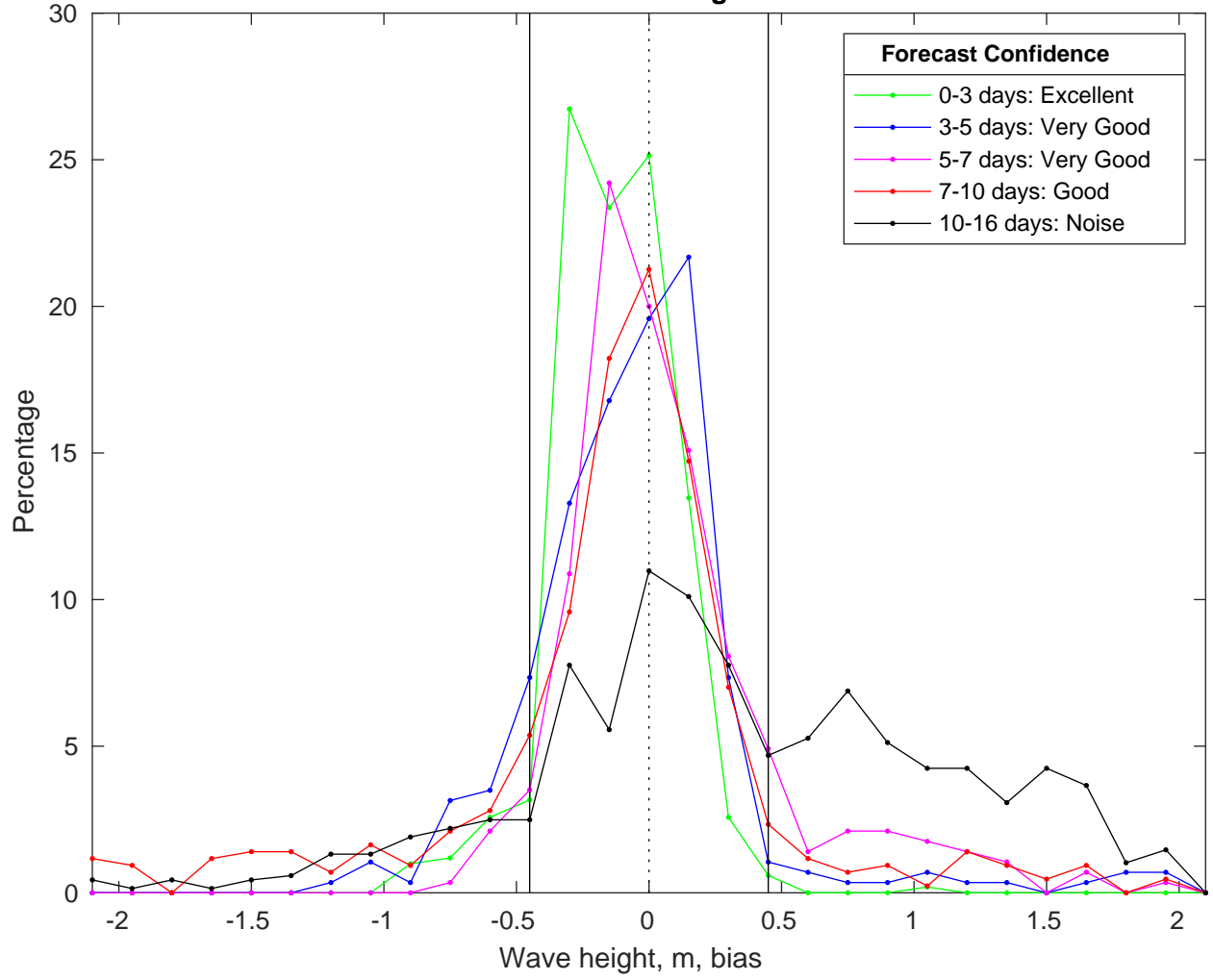
NDBC 46028 vs GFSWaves Bias Histogram: 03-Feb-2025
