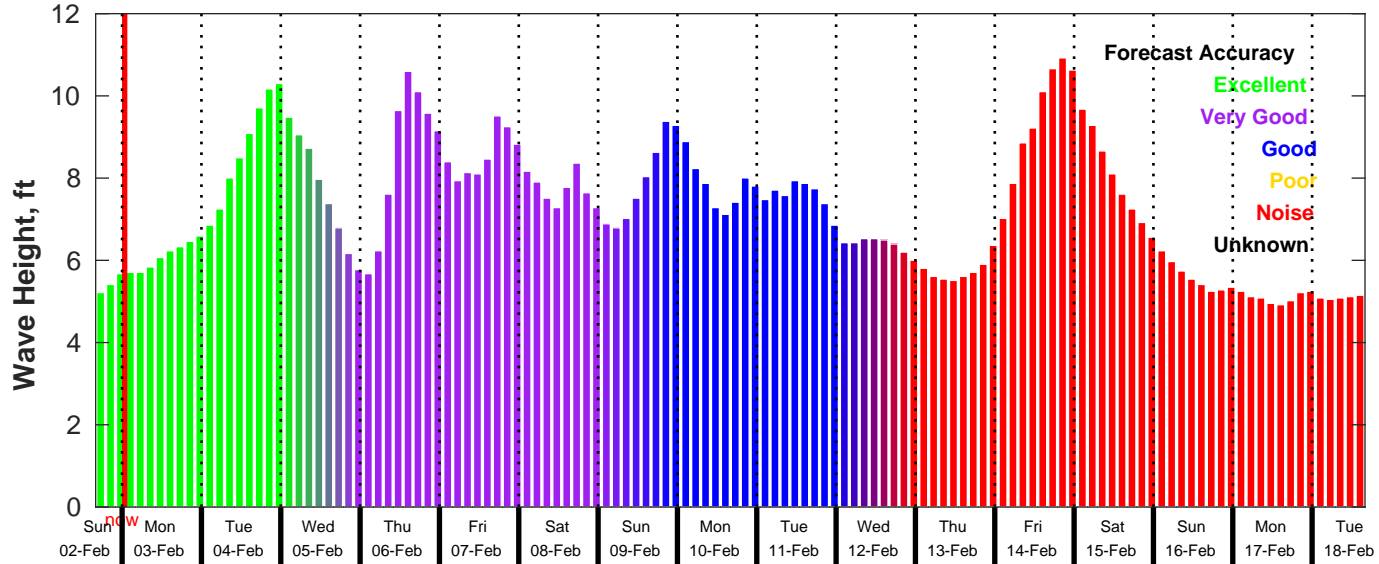
GFS Wave Forecast for NDBC 46028 from 02-Feb-2025 16:00:00 to 18-Feb-2025 16:00:00
