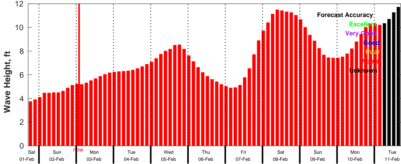
CMEMS Wave Forecast for NDBC 46053 from 01-Feb-2025 17:00:00 to 11-Feb-2025 17:00:00
