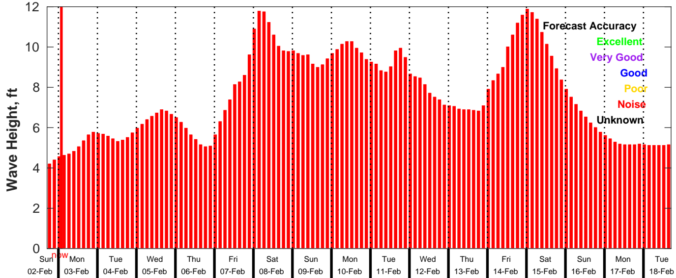
GFS Wave Forecast for NDBC 46053 from 02-Feb-2025 17:00:00 to 18-Feb-2025 17:00:00
