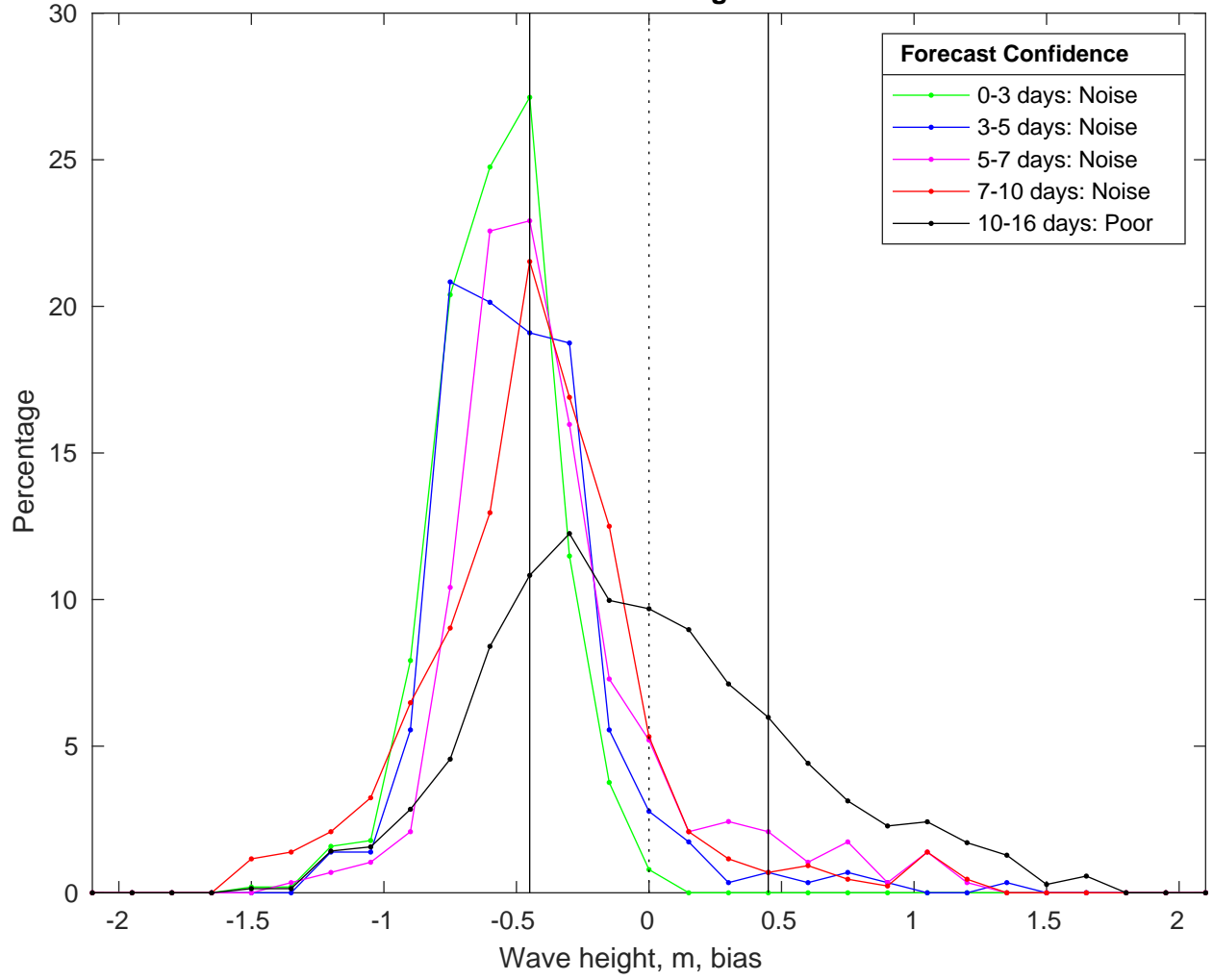
NDBC 46054 vs GFSWaves Bias Histogram: 03-Feb-2025
