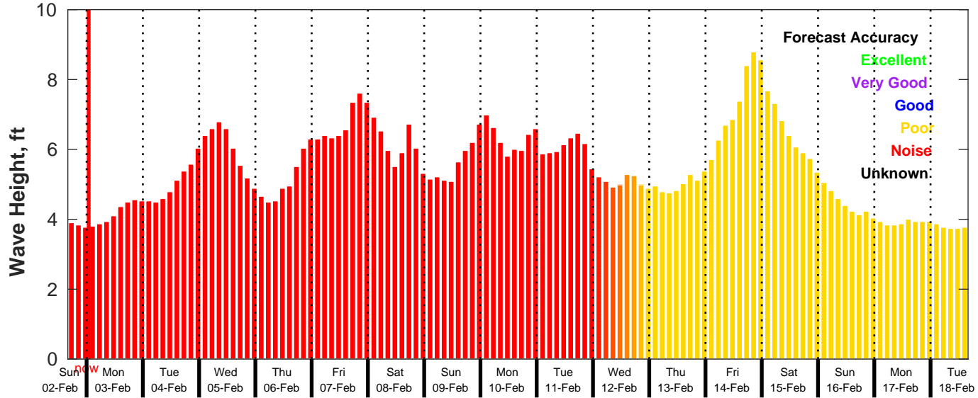
GFS Wave Forecast for NDBC 46054 from 02-Feb-2025 16:00:00 to 18-Feb-2025 16:00:00
