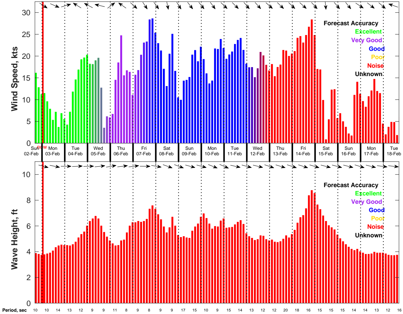
Wind & Wave Forecast for NDBC 46054 from 02-Feb-2025 16:00:00 to 18-Feb-2025 16:00:00
