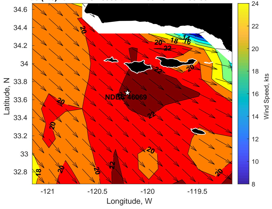
Winds (kts) for NDBC 46069 at 12-Dec-2024 21:00:00
