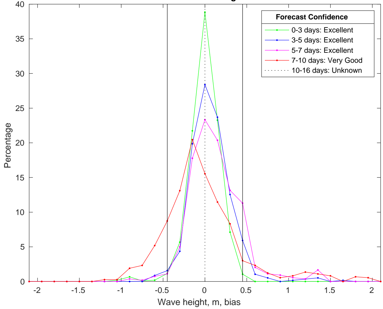
NDBC 46069 vs CMEMSWaves Bias Histogram: 03-Feb-2025
