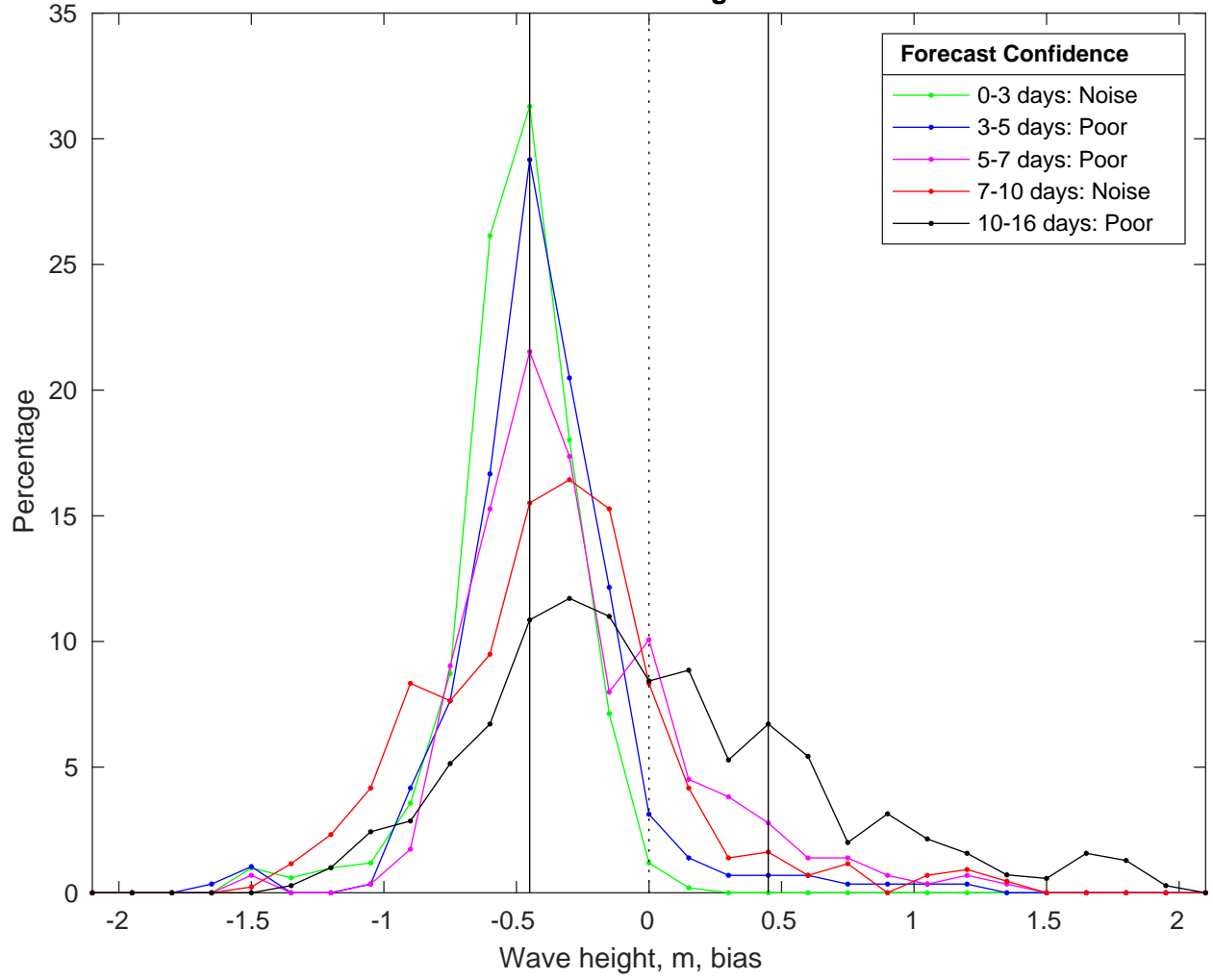
NDBC 46069 vs GFSWaves Bias Histogram: 03-Feb-2025
