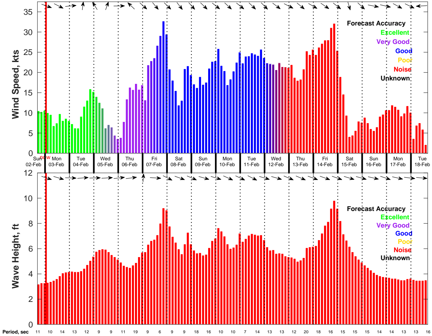
Wind & Wave Forecast for NDBC 46069 from 02-Feb-2025 16:00:00 to 18-Feb-2025 16:00:00
