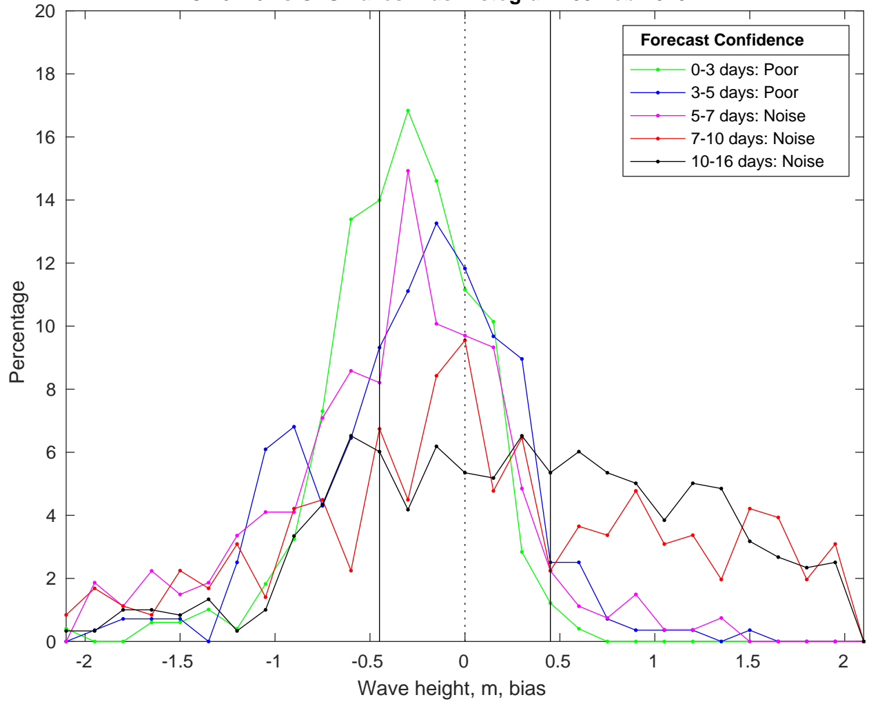
NDBC 46246 vs GFSWaves Bias Histogram: 03-Feb-2025
