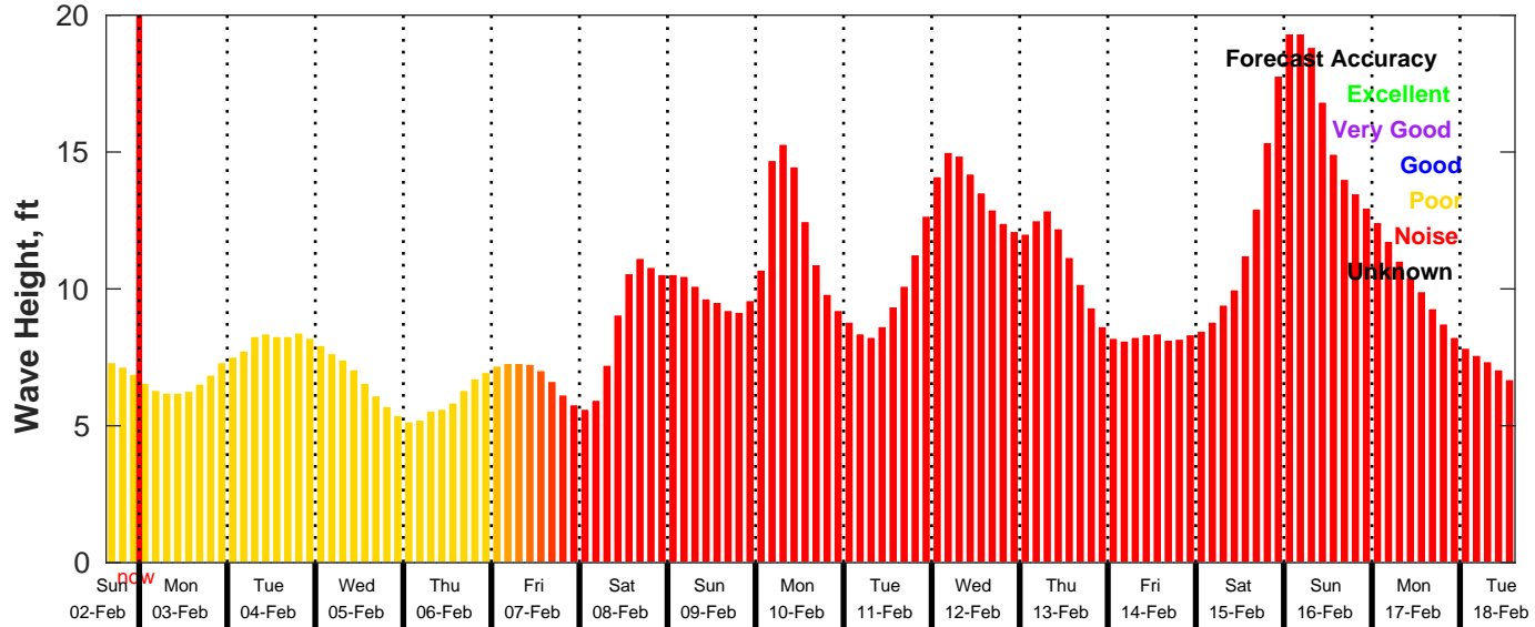
GFS Wave Forecast for NDBC 46246 from 02-Feb-2025 15:00:00 to 18-Feb-2025 15:00:00
