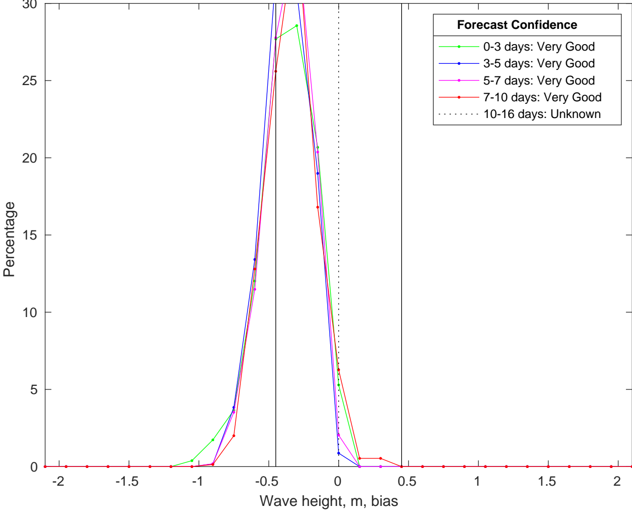
NDBC 51209 vs CMEMSWaves Bias Histogram: 03-Feb-2025
