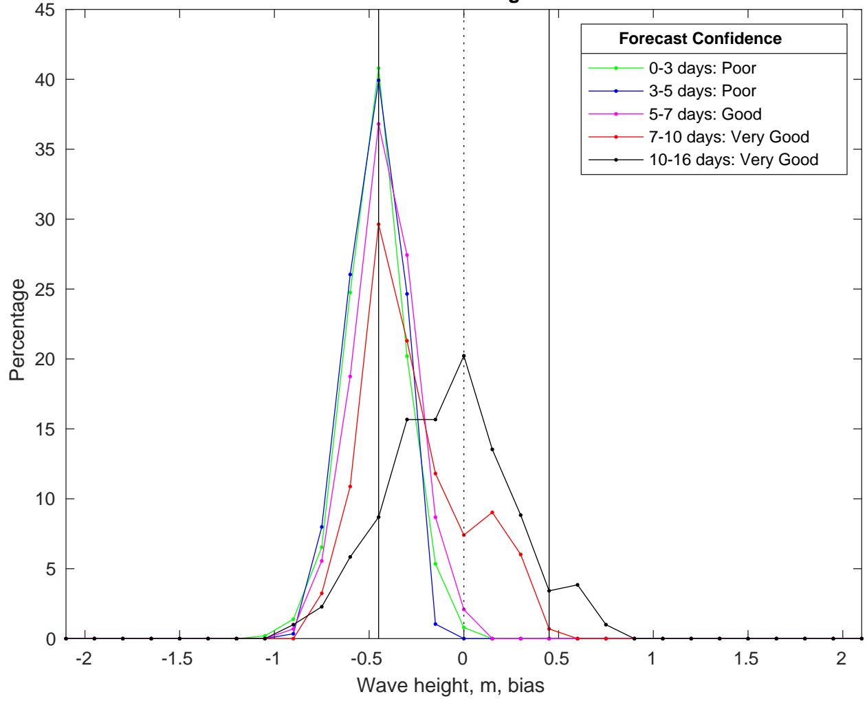
NDBC 51209 vs GFSWaves Bias Histogram: 03-Feb-2025
