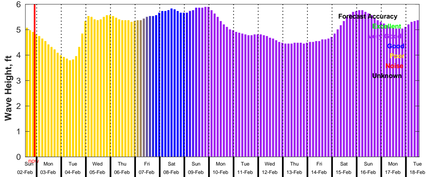
GFS Wave Forecast for NDBC 51209 from 02-Feb-2025 13:00:00 to 18-Feb-2025 13:00:00
