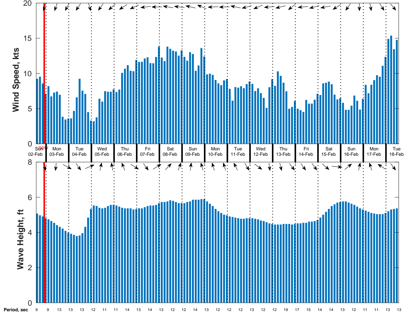
Wind & Wave Forecast for NDBC 51209 from 02-Feb-2025 13:00:00 to 18-Feb-2025 13:00:00
