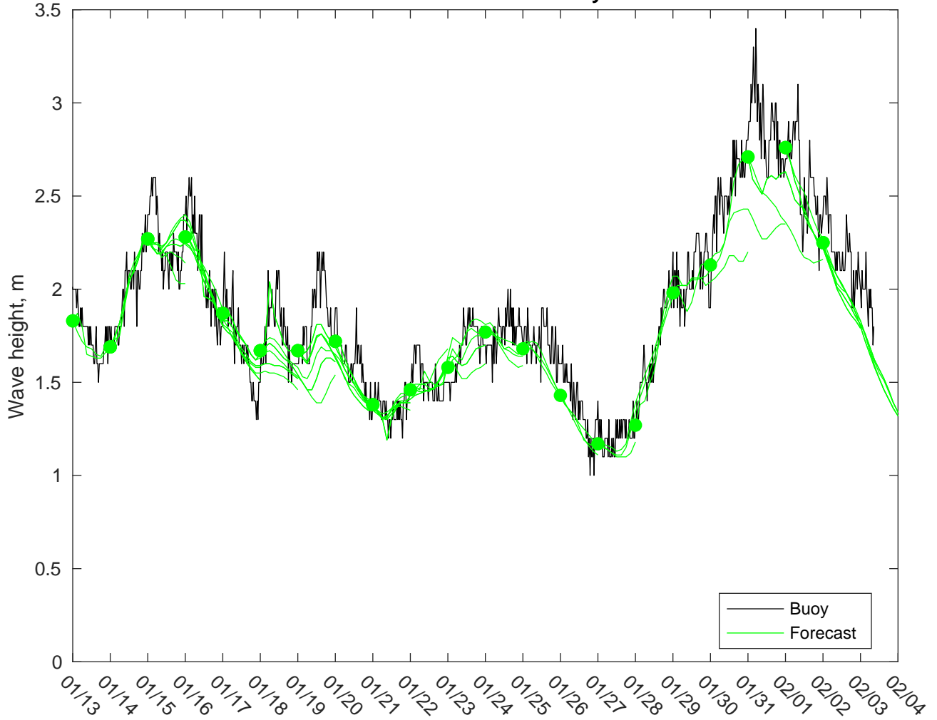
NDBC 52211 vs CMEMSWaves: 0 to 3 day forecast
