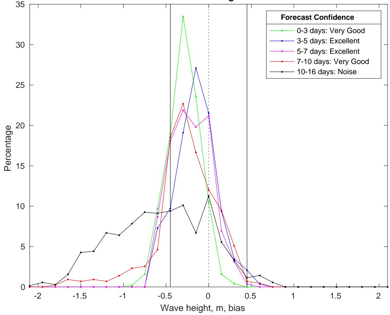
NDBC 52212 vs GFSWaves Bias Histogram: 03-Feb-2025
