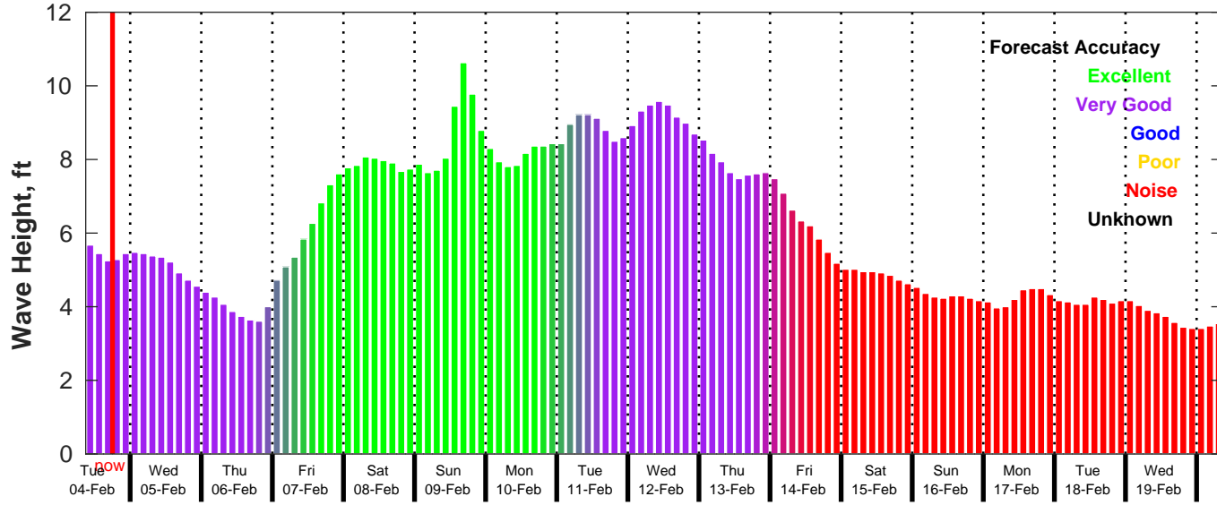
GFS Wave Forecast for NDBC 52212 from 03-Feb-2025 09:00:00 to 19-Feb-2025 09:00:00
