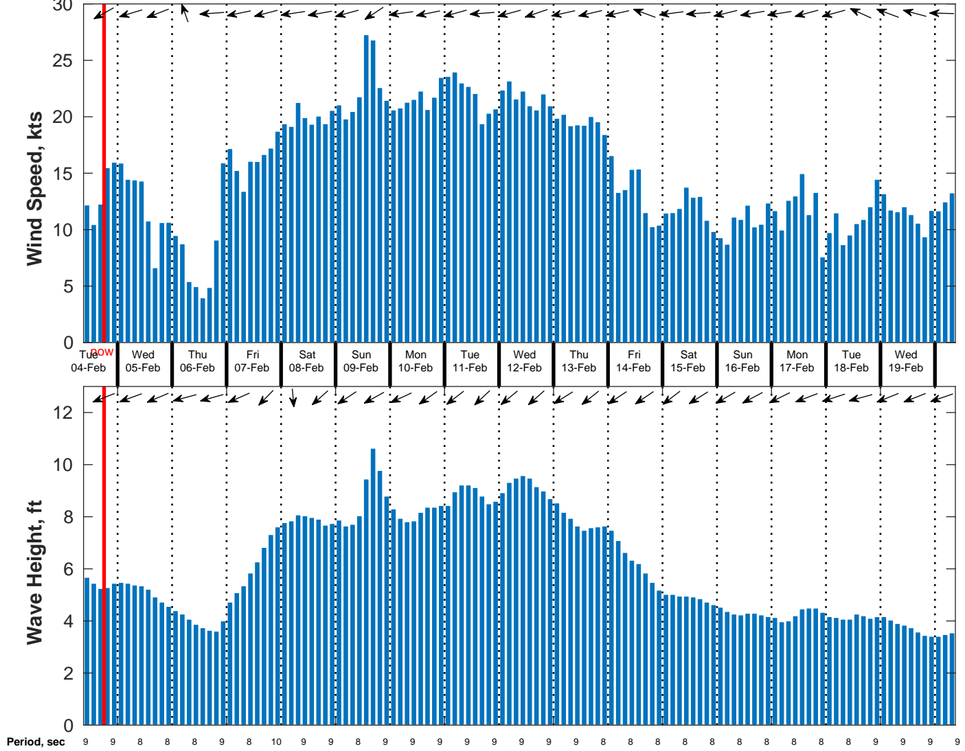
Wind & Wave Forecast for NDBC 52212 from 03-Feb-2025 09:00:00 to 19-Feb-2025 09:00:00
