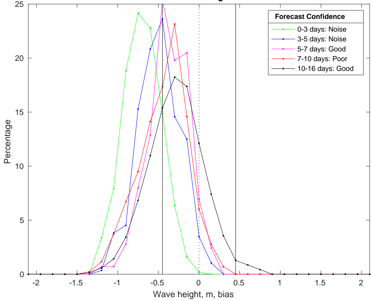
NDBC 52213 vs GFSWaves Bias Histogram: 03-Feb-2025
