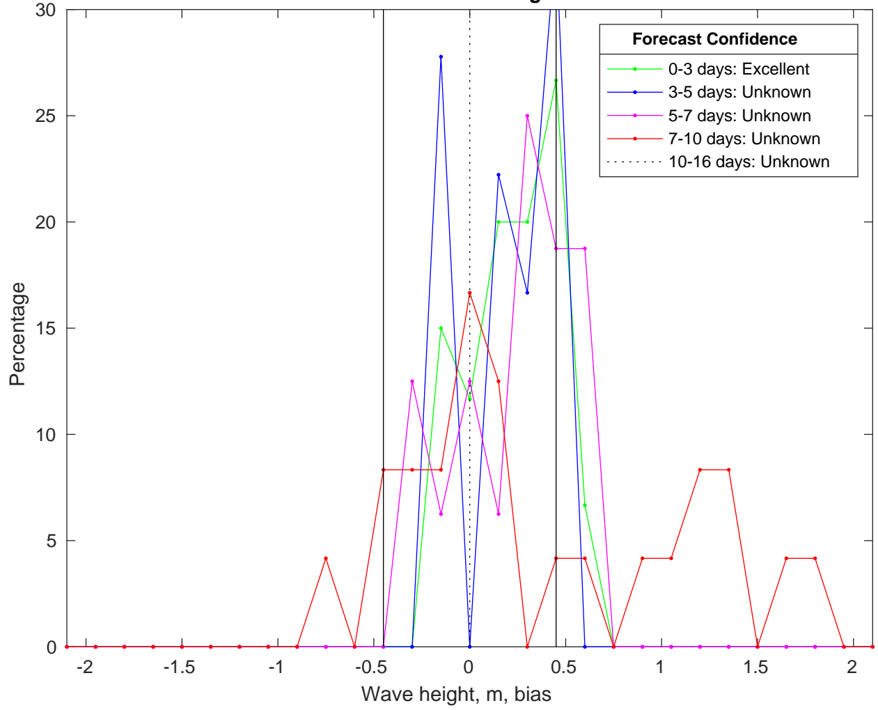
NDBC 62305 vs CMEMSWaves Bias Histogram: 03-Feb-2025
