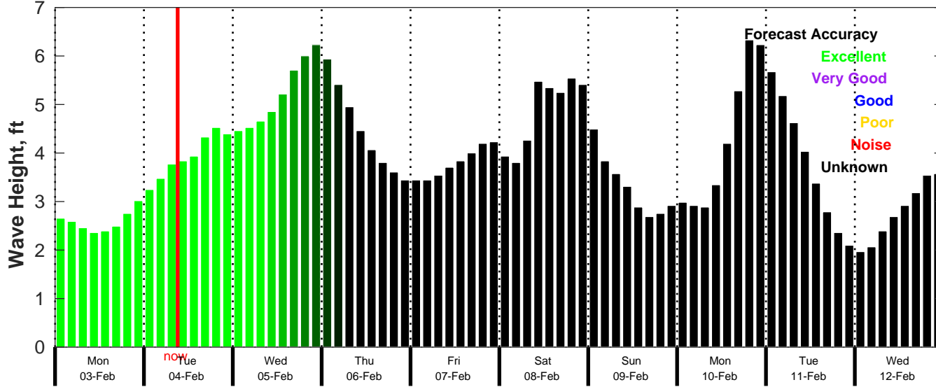
CMEMS Wave Forecast for NDBC 62305 from 02-Feb-2025 00:00:00 to 12-Feb-2025 00:00:00
