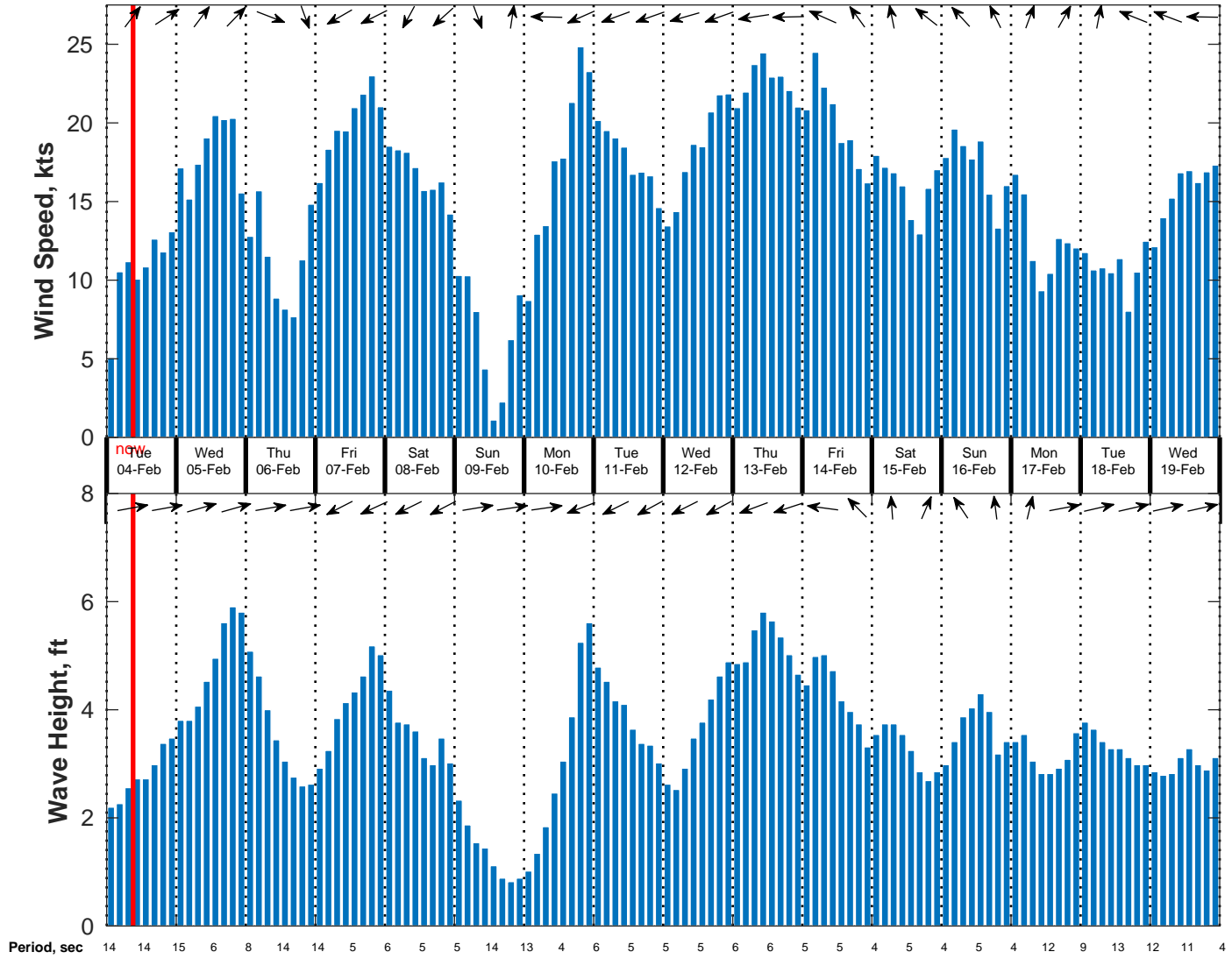
Wind & Wave Forecast for NDBC 62305 from 03-Feb-2025 00:00:00 to 19-Feb-2025 00:00:00
