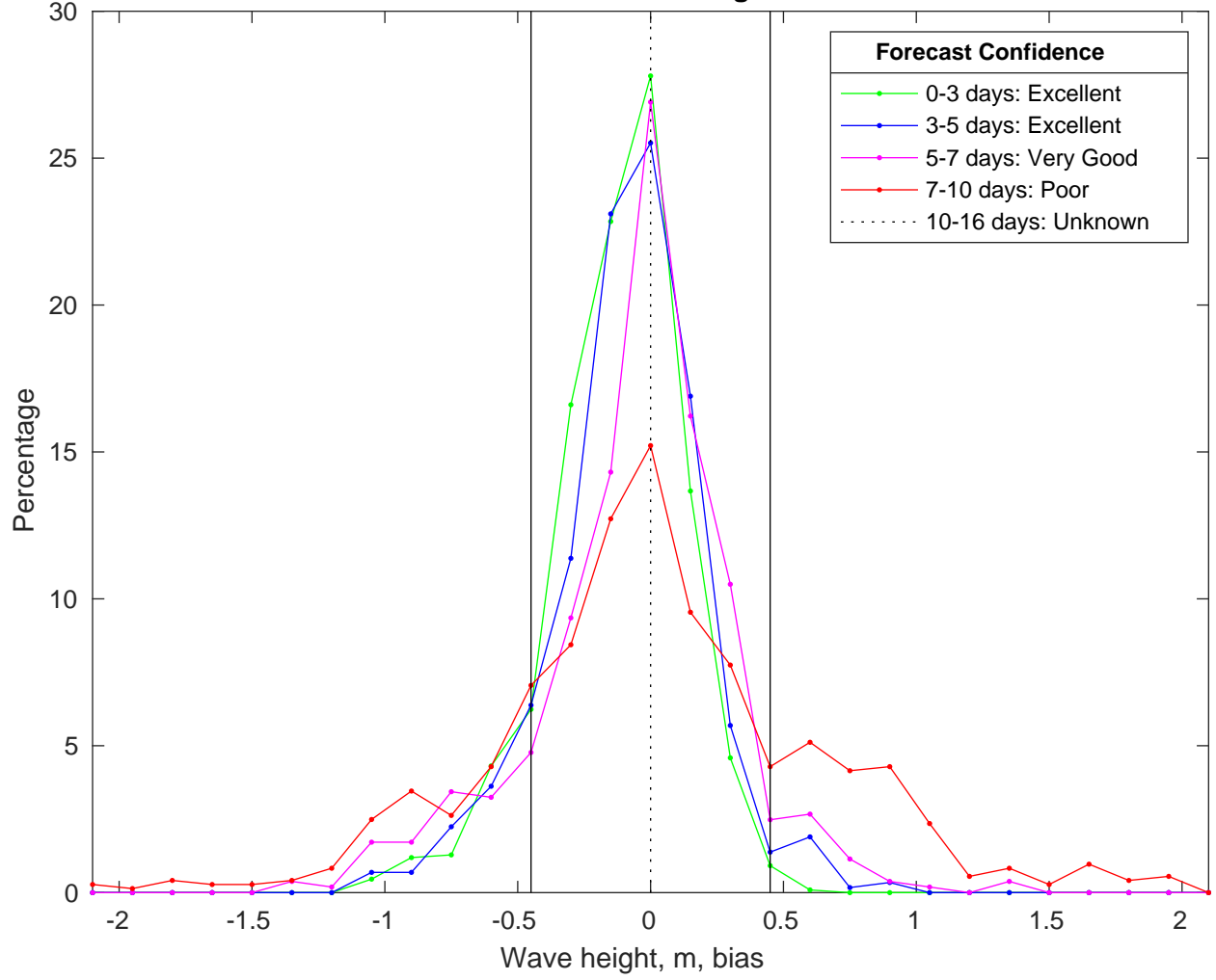
NDBC 41004 vs CMEMSWaves Bias Histogram: 04-Feb-2025
