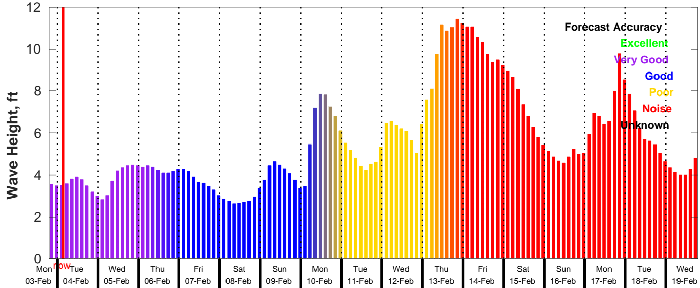
GFS Wave Forecast for NDBC 41004 from 03-Feb-2025 19:00:00 to 19-Feb-2025 19:00:00
