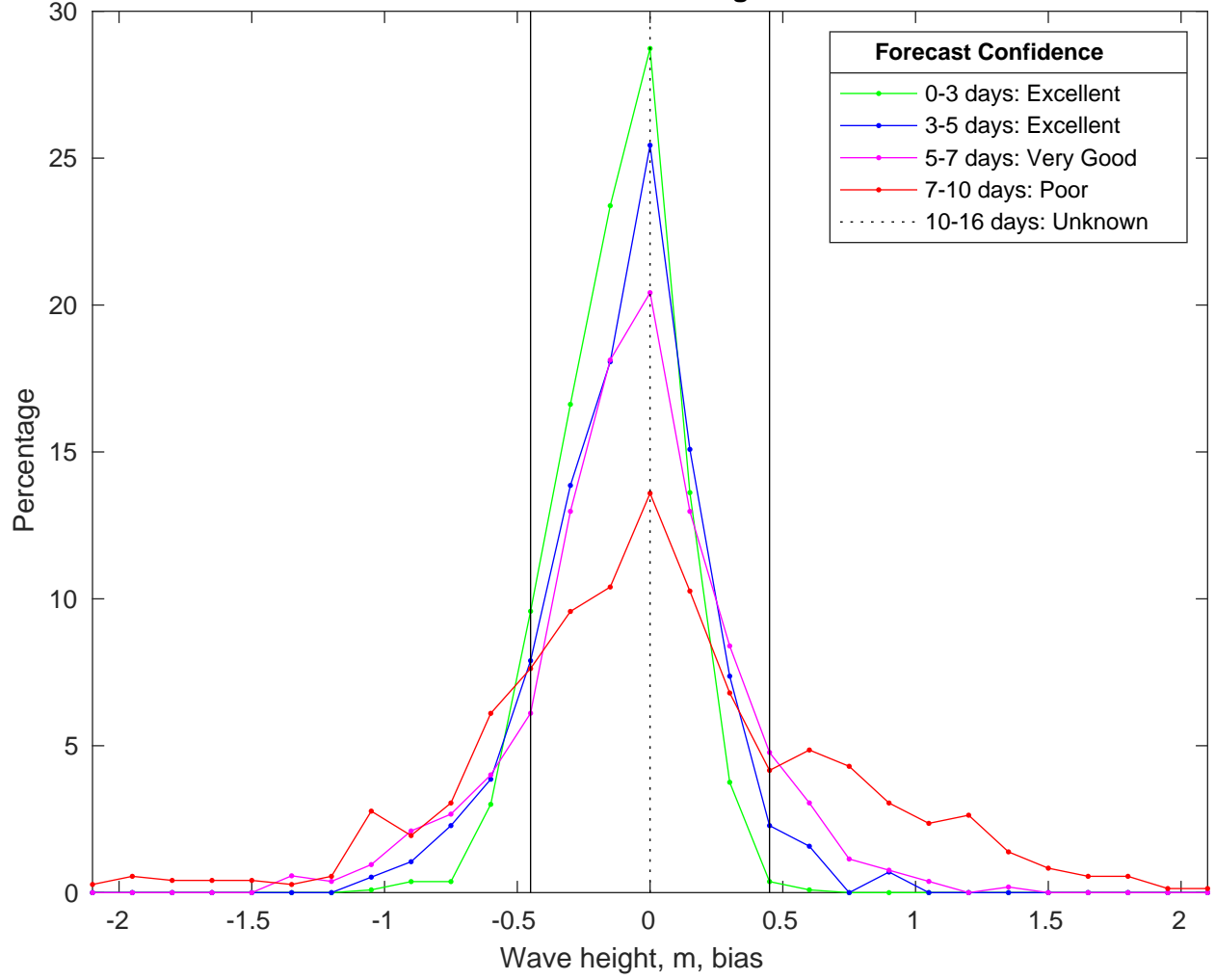
NDBC 41013 vs CMEMSWaves Bias Histogram: 04-Feb-2025
