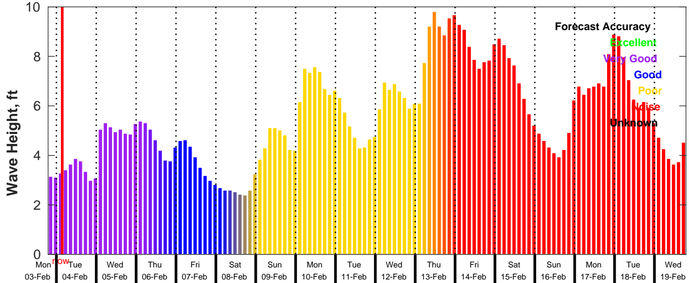
GFS Wave Forecast for NDBC 41013 from 03-Feb-2025 19:00:00 to 19-Feb-2025 19:00:00
