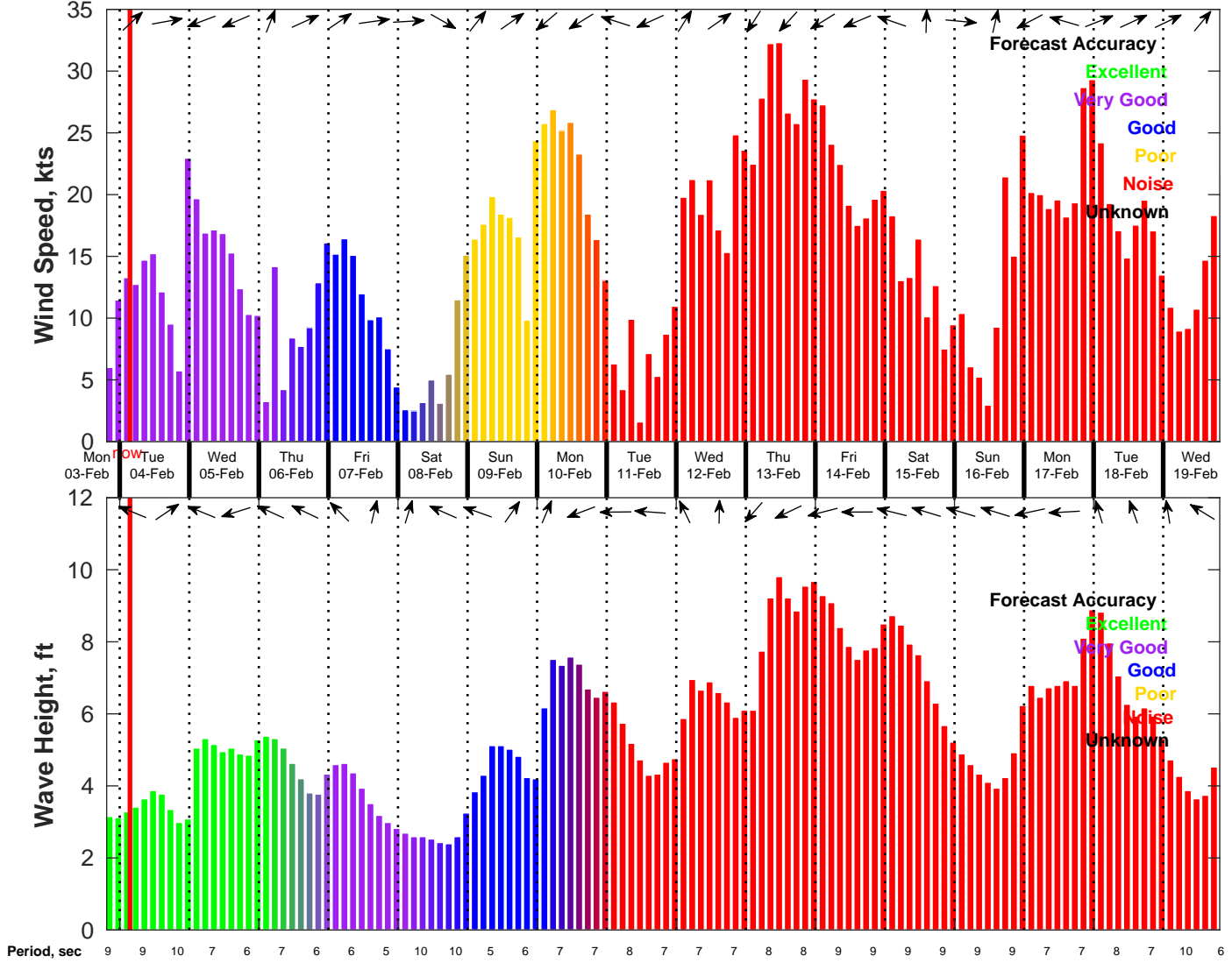
Wind & Wave Forecast for NDBC 41013 from 03-Feb-2025 19:00:00 to 19-Feb-2025 19:00:00
