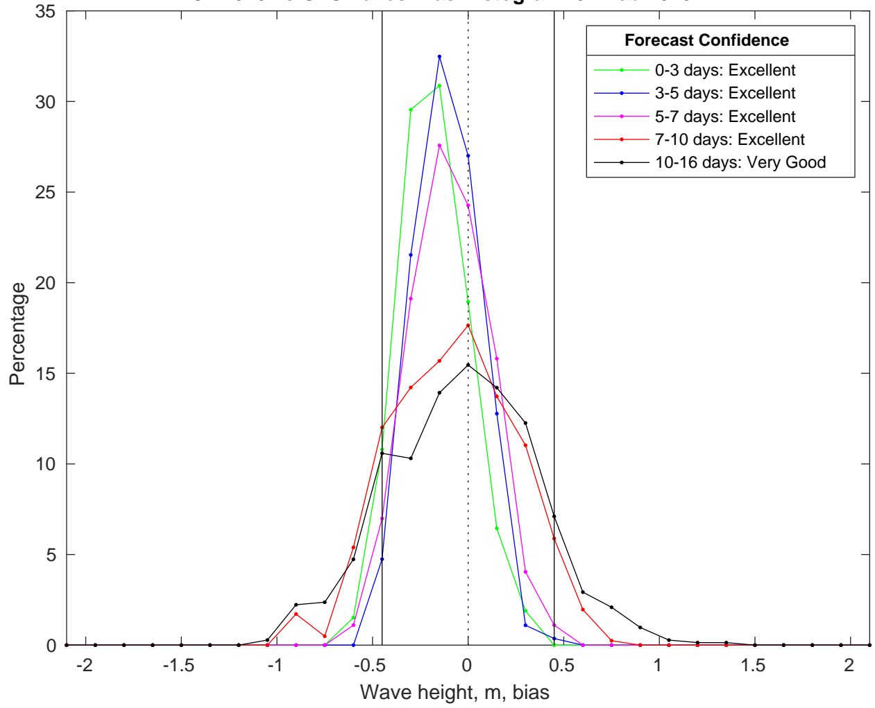
NDBC 41040 vs GFSWaves Bias Histogram: 04-Feb-2025
